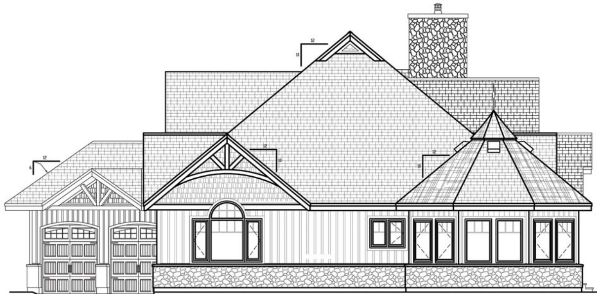
LEFT ELEVATION
